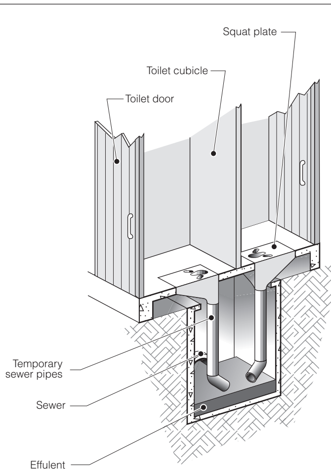
Figure 6.12. Temporary toilet block over existing sewer
