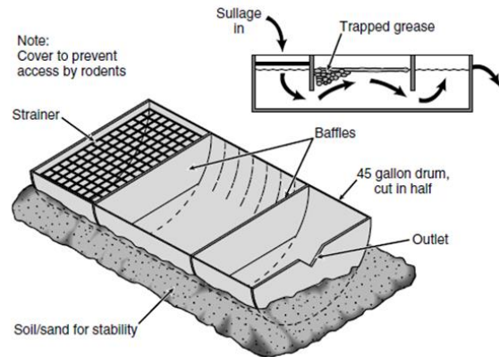
Figure 6 A simple grease trap. From Engineering in Emergencies (RedR, 2002)
