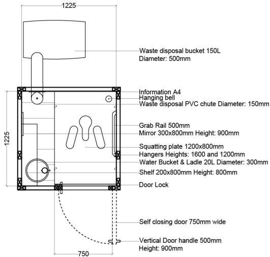
Latrine Cubicle Plan 1:50
