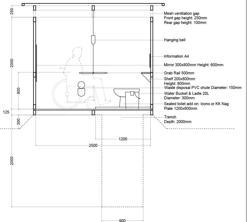
Latrine Cubicle PRM Section 1:50
