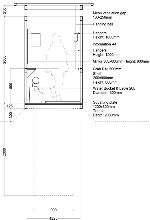
Latrine Cubicle Section 1:50
