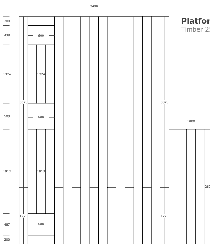
TL_Platform Floor Boards
