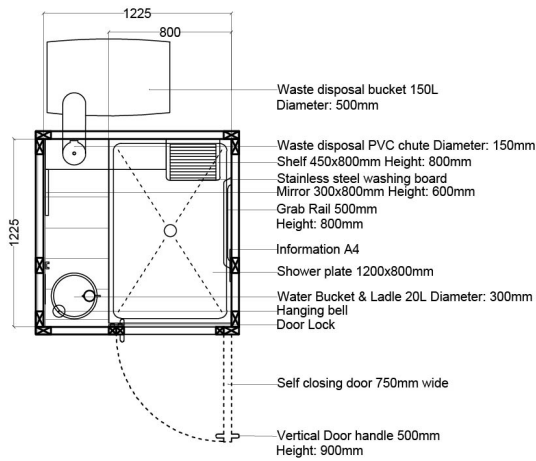
Bathing Cubicle Plan 1:50
