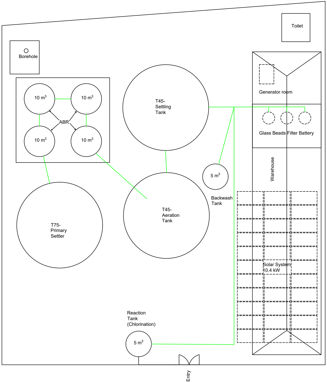
Figure: Layout of FSM Plant at Camp 19
