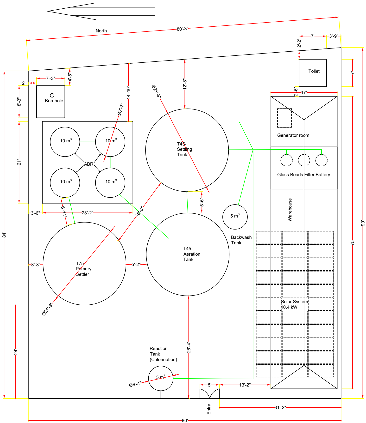
Figure: Layout of FSM Plant at Camp 19
